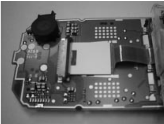
PHOTO 2.10 Disassemble Control Board Assy – STEP 2
