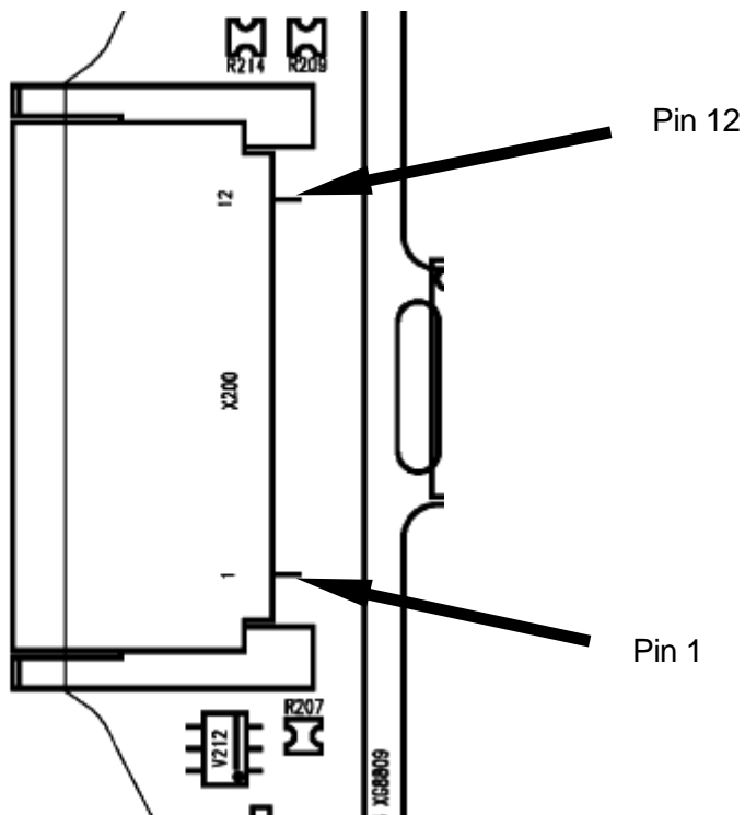
Figure 2: X35 Bottom Connector Placement (Top View)
