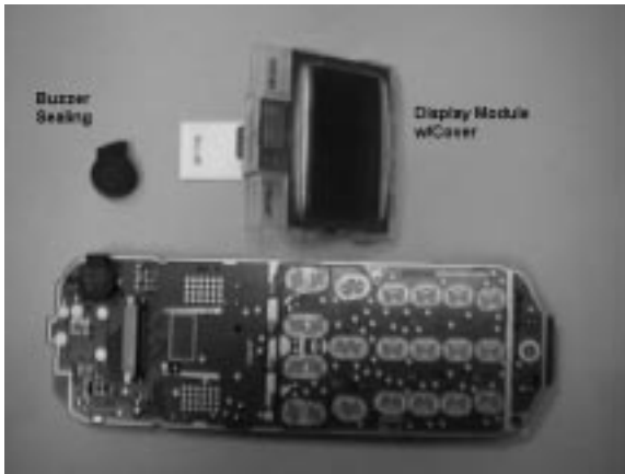
PHOTO 2.11 Disassemble Control Board Assy – STEP 2
