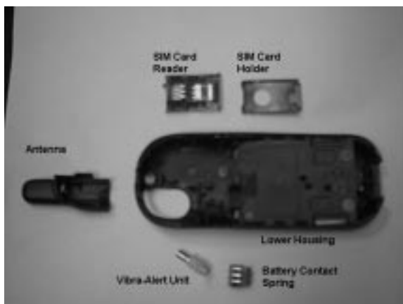
PHOTO 2.8 Disassembly Lower Housing – STEP 2
