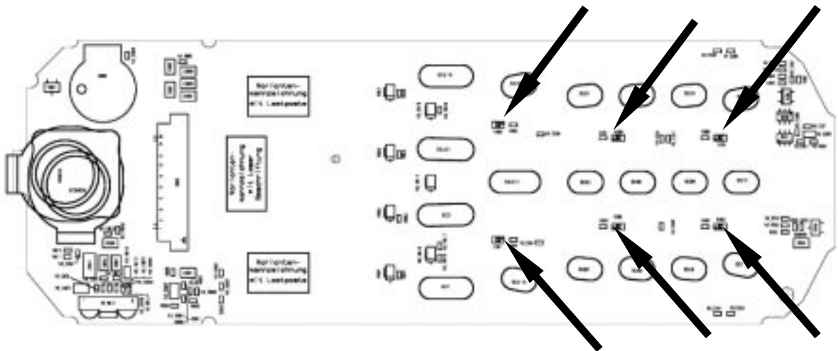
Figure 2: X35 keyboard LED placement and polarity (top view)
