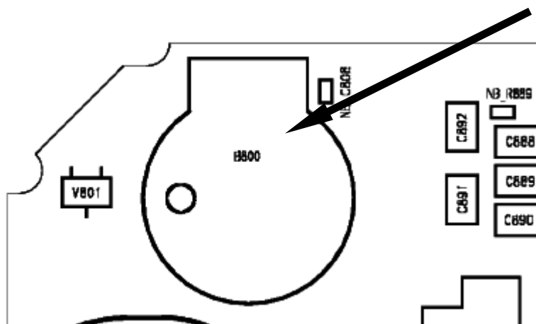
Figure 2: X35 Ringer (B800) Placement (Top View)
