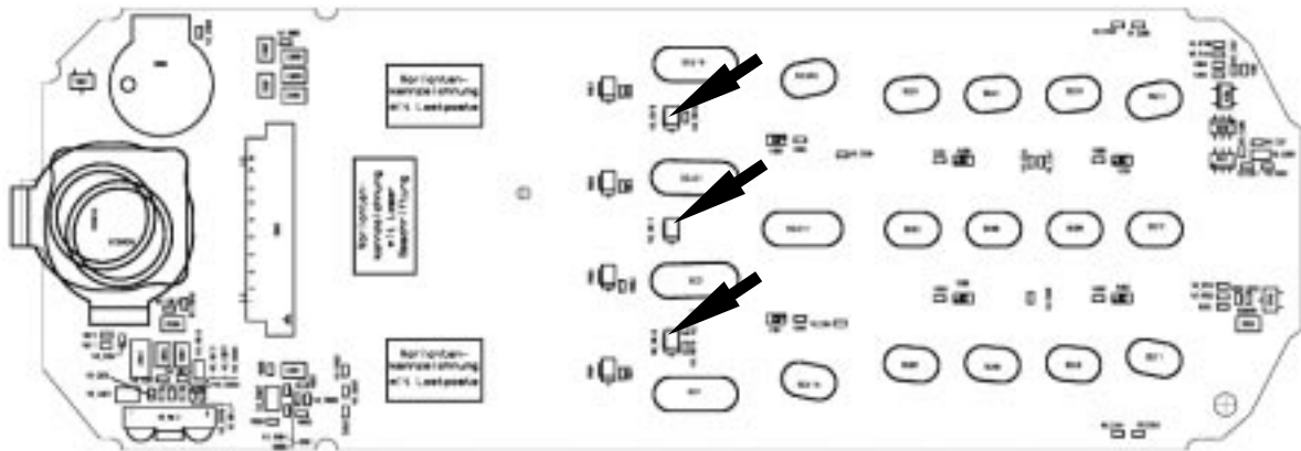
Figure 3: S35 board display LED side
